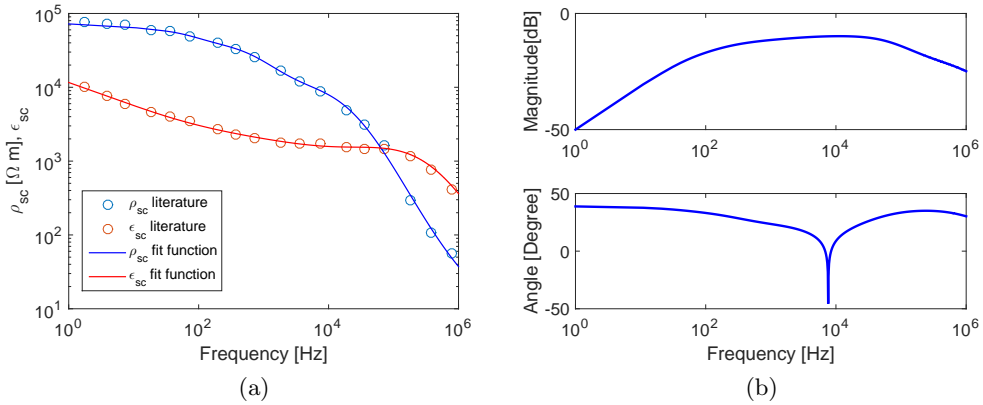
Fig. 2: a. The resistivity and dielectric constant of epidermal stratum corneum by [30] and the polynomial functions fitted by us on the experimental data points. b. Bode plot of the transfer function \frac{V_{sc}}{V} .
