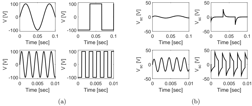
Fig. 3: a. The input voltage signals used in Matlab/Simulink simulations; sinusoidal and square signals at 15 Hz (first row) and 480 Hz (second row). b. The resulting voltage on the stratum corneum, V_{sc} , for the four cases.
