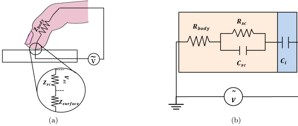
Fig. 1: a. Equivalent circuit model of human finger on a touch surface. b. The simplified equivalent circuit model of human finger on a touch surface.
